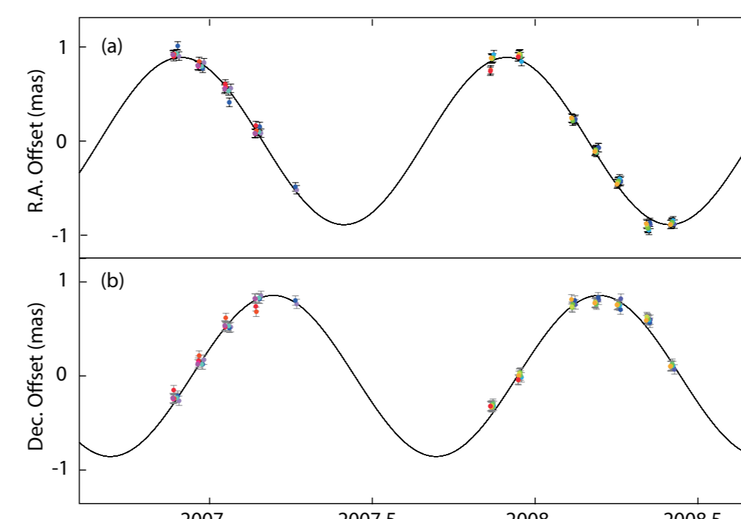
Fig.3. R UMa, parallactic motion. (Nakagawa et al. in prep.)
