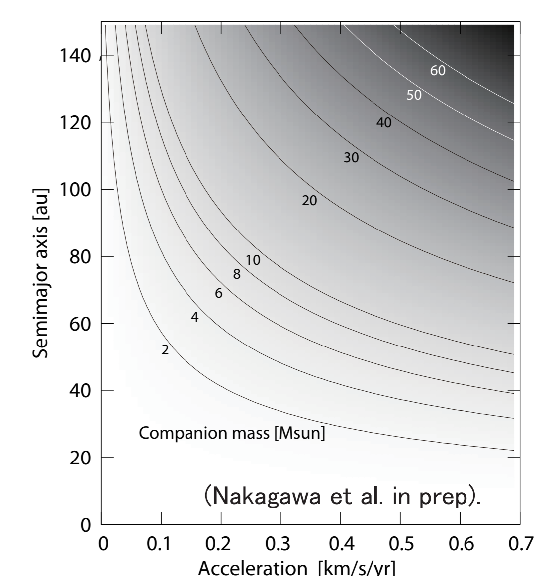
Fig.6. Binary orbit semimajor axis, acceleration of binary motion and companion mass.
