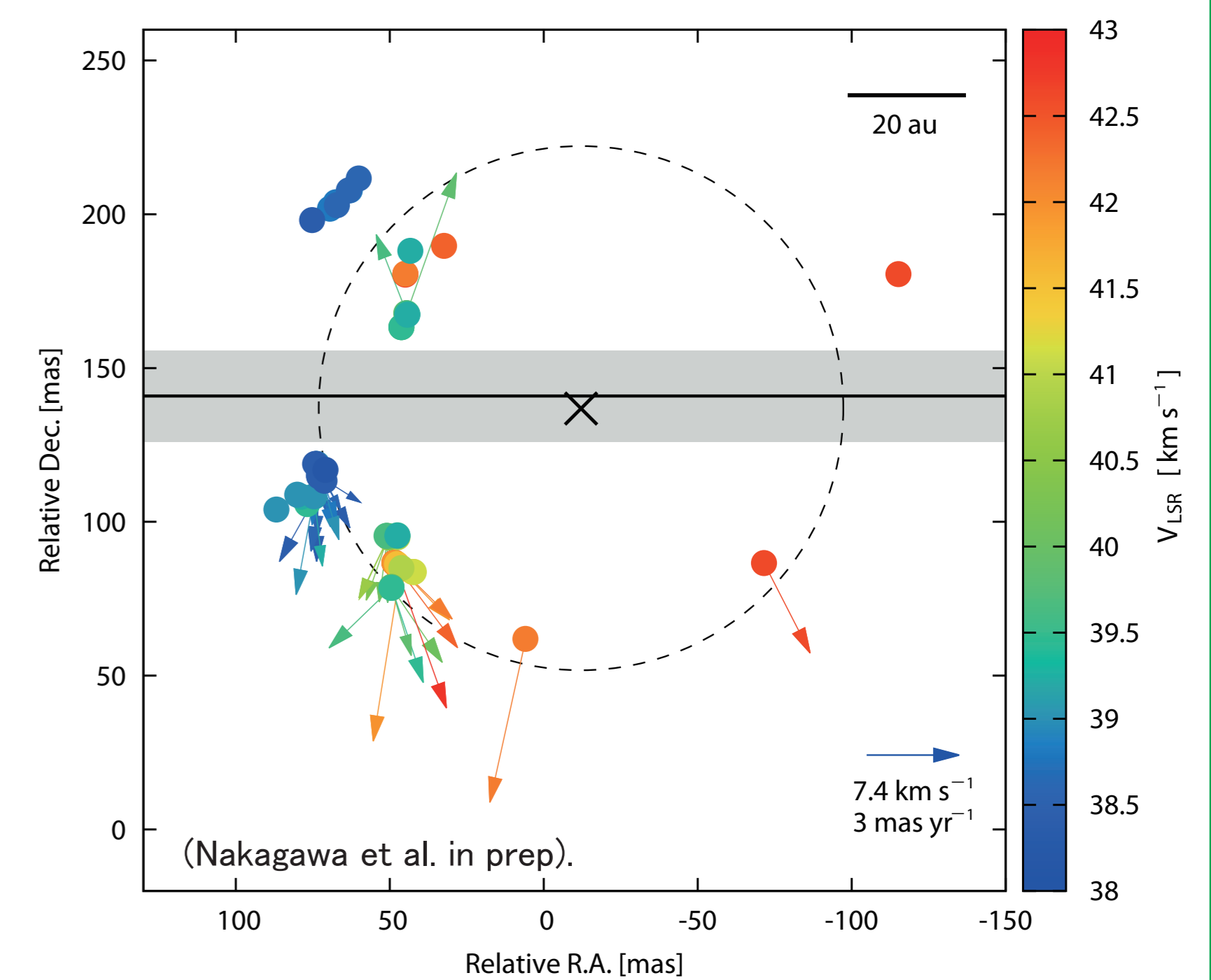
Fig.4. Distribution of water masers in R UMa. A cross mark indicate an estimated star position.
