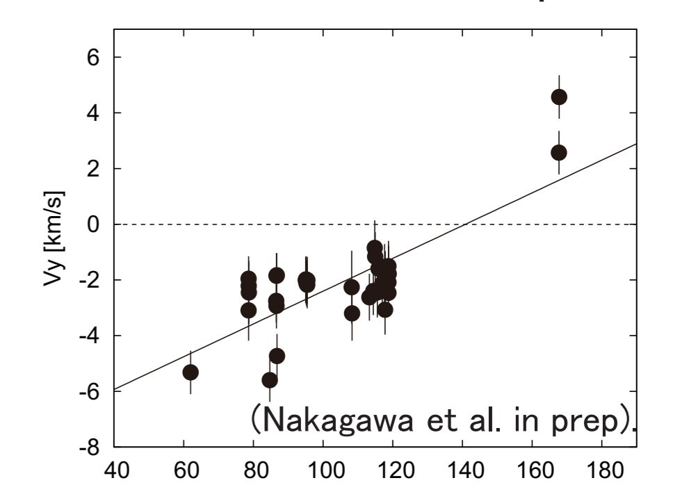
Fig.5. Internal motion velocity gradient of maser spots along DEC.
