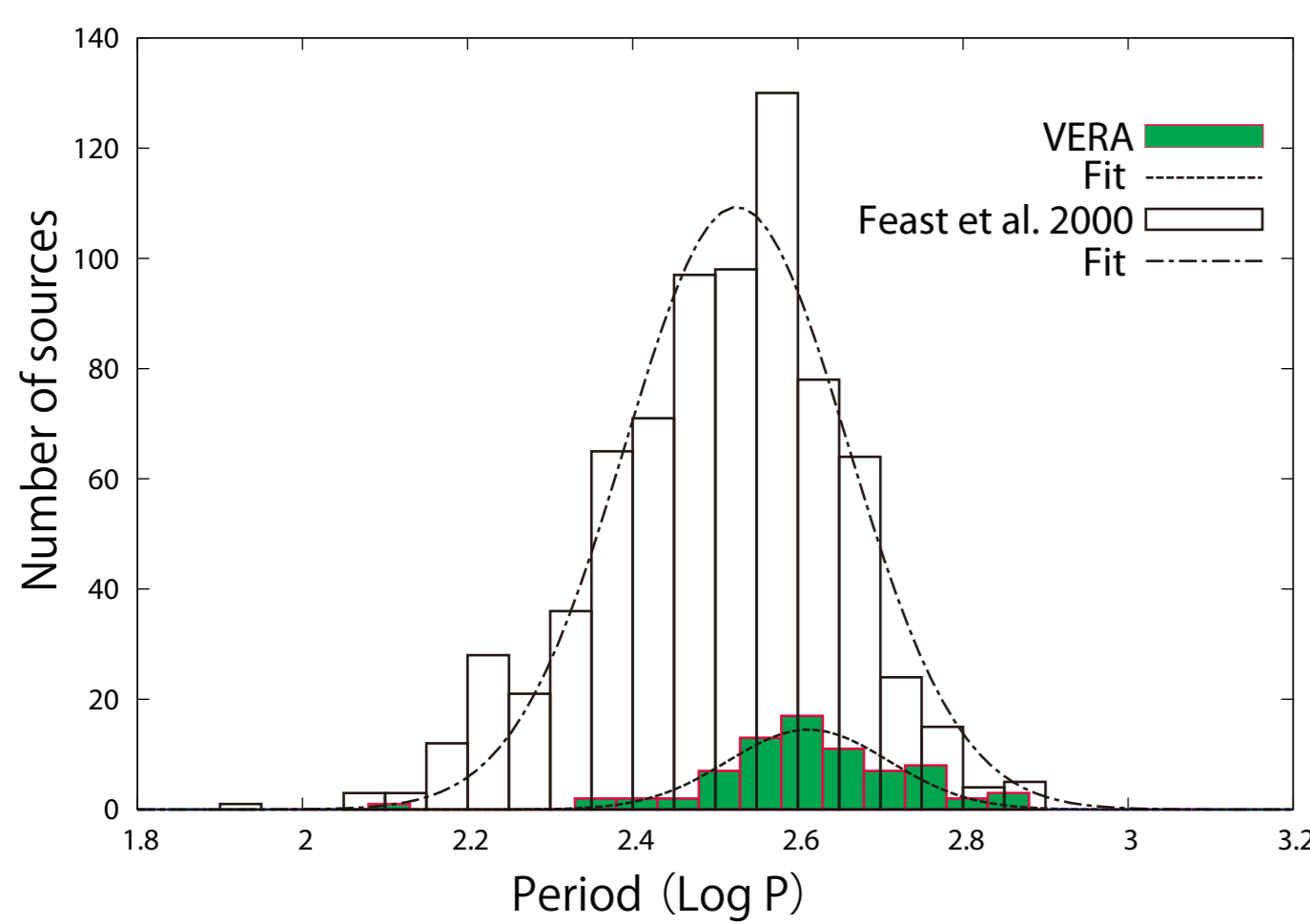
Fig.1. Period distribution of Mira variables in Feast et al. (2000) (white) and our targets (green).
